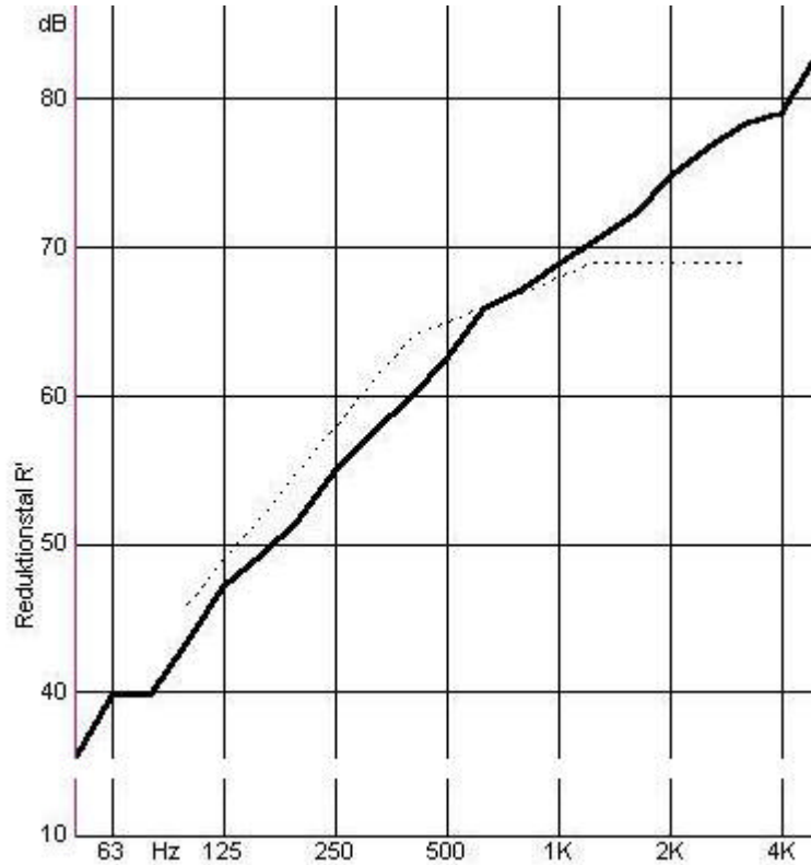
Figure 4. The same slab and access floor with one additional parquet layer (9 kg/m 2 ), measured in situ with suppressed flanking transmission. R'_w+C_{50-3150} 65 (+0) dB.
